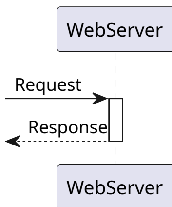
Figure 78: Example of a sequence diagram lifeline
